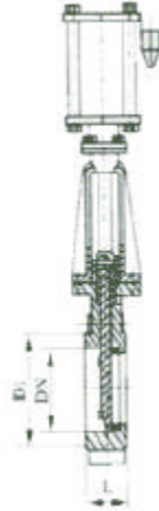
主要外型及连接尺寸 Main External And Connecting Dimensions(mm)
