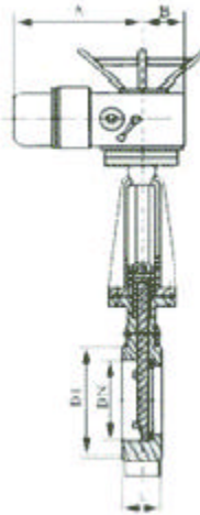
主要外型及连接尺寸 Main External And Connecting Dimensions(mm)
