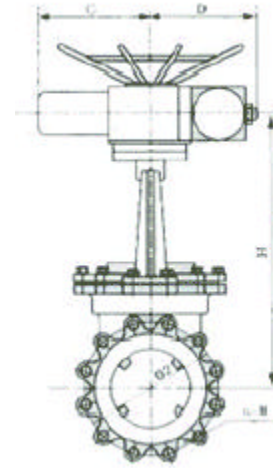
主要外型及连接尺寸 Main External And Connecting Dimensions(mm)
