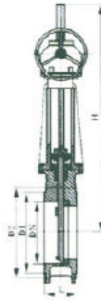
主要外型及连接尺寸 Main External And Connecting Dimensions(mm)
