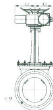
主要外型及连接尺寸 Main External And Connecting Dimensions(mm)
