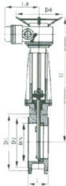
主要外型及连接尺寸 Main External And Connecting Dimensions(mm)
