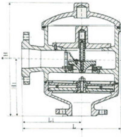
HXF7Y型带接管阻火呼出阀
