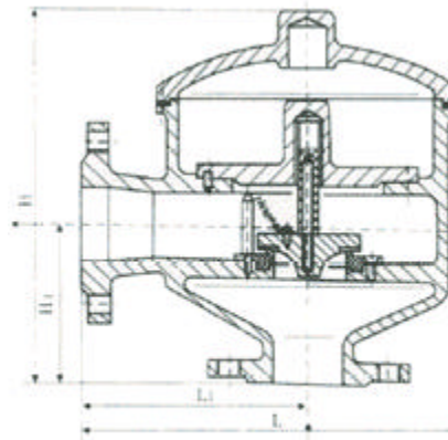
HX7Y型带接管呼出阀
