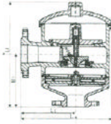
HXF7型带接管阻火呼出阀 DN50-300
