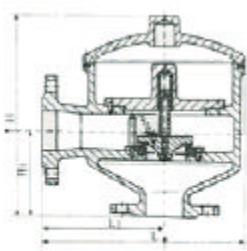
HX7型带接管呼出阀 DN50-300
