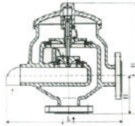
HX4型带呼出接管呼吸阀 DN50-250
