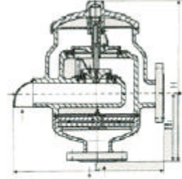
HXF4型带呼出接管阻火呼吸阀 DN50-250
