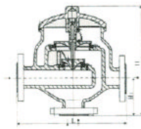
HX2型带双接管呼吸阀 DN50-250
