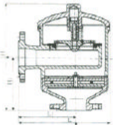
HXF8型带接管阻火吸入阀 DN50-250
